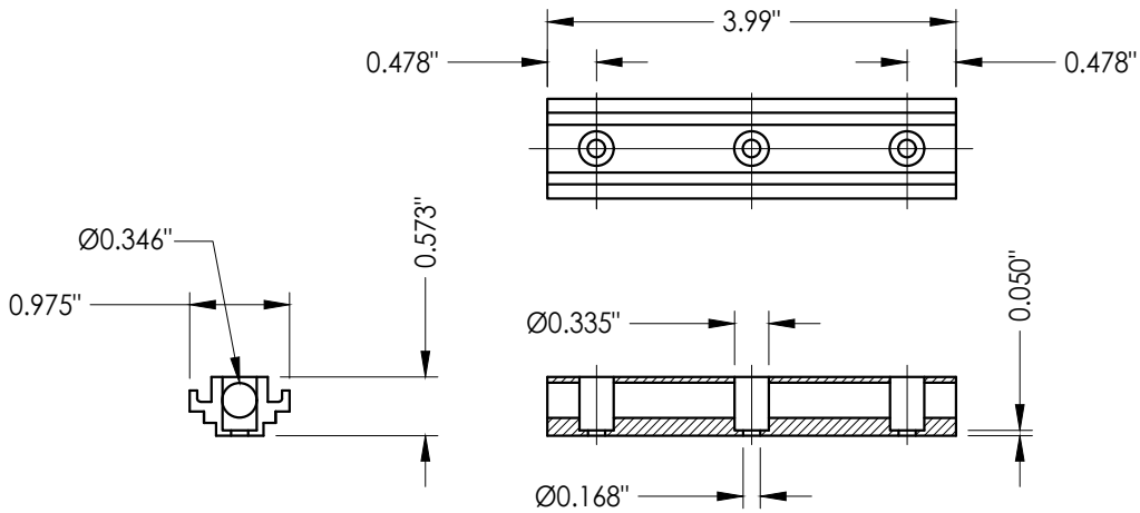
CONCEALED STIFFENER
